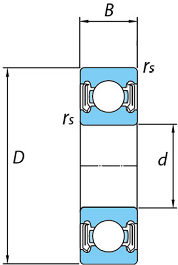
Non-contact sealed type (LLB)
