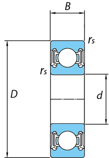
Contact sealed type (LLU)
